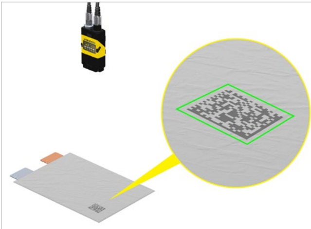
A DataMan 260 image-based barcode reader reads stretched DataMatrix codes on a pouch's surface.
