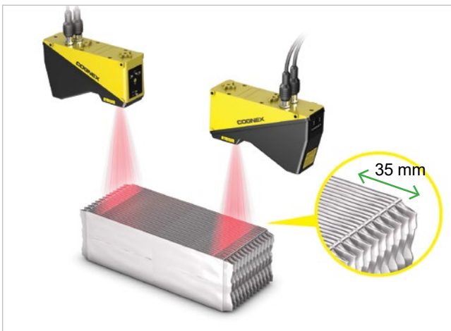
Two DS1000 3D laser displacement sensors measure the profile of cell batteries stacked inside a module.
