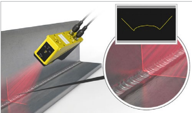
DS1000 3D laser displacement sensors inspect the welding seams of metal components before they are painted.
