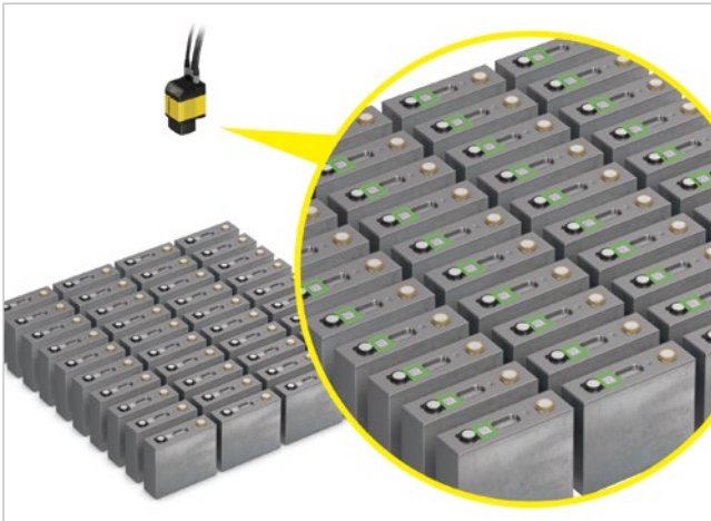
The DataMan 470 barcode reader reads a large array of codes on battery modules during testing.
