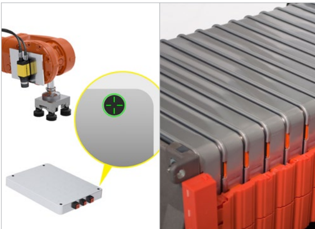
The In-Sight 8000 vision system guides the final assembly of modules and cable connectors into a pack.
