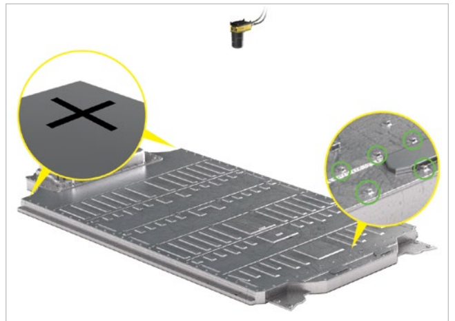
The In-Sight 9912 vision system inspects the final battery pack for completeness and fixtures it for robotic placement.
