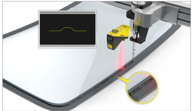
The In-Sight Laser Profiler measures glue bead volume to ensure the correct amount of glue has been dispensed.
