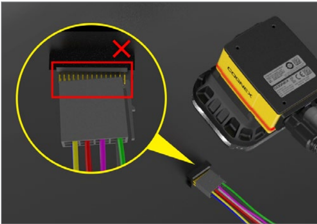
In-Sight 7000 vision systems confirm that wiring harnesses are properly seated.
