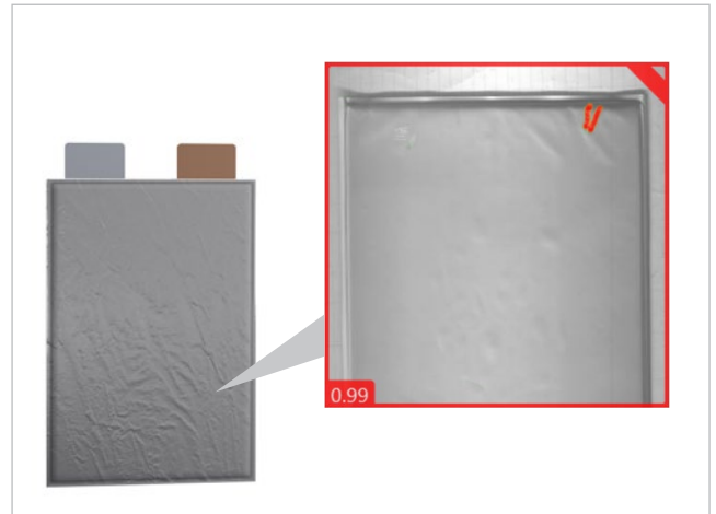
Cognex Deep Learning identifies surface defects, like bubbles and wrinkles, on a pouch's surface.
